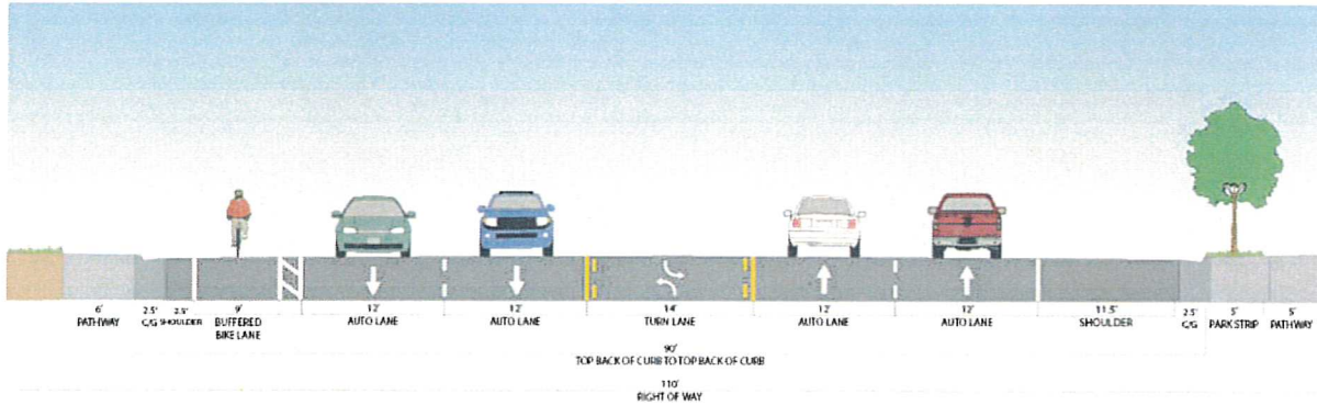
Figure 34 – 110-Foot Major Arterial
